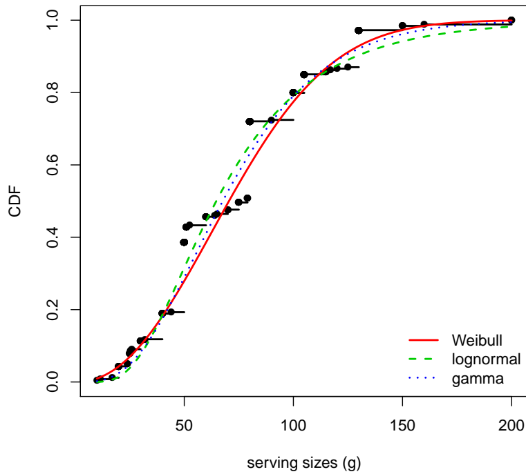
Figure 6: Comparison of CDF plots of various distributions fitted on continuous data (Weibull, gamma and lognormal distributions fitted to serving sizes from the “ground beef” data set)
